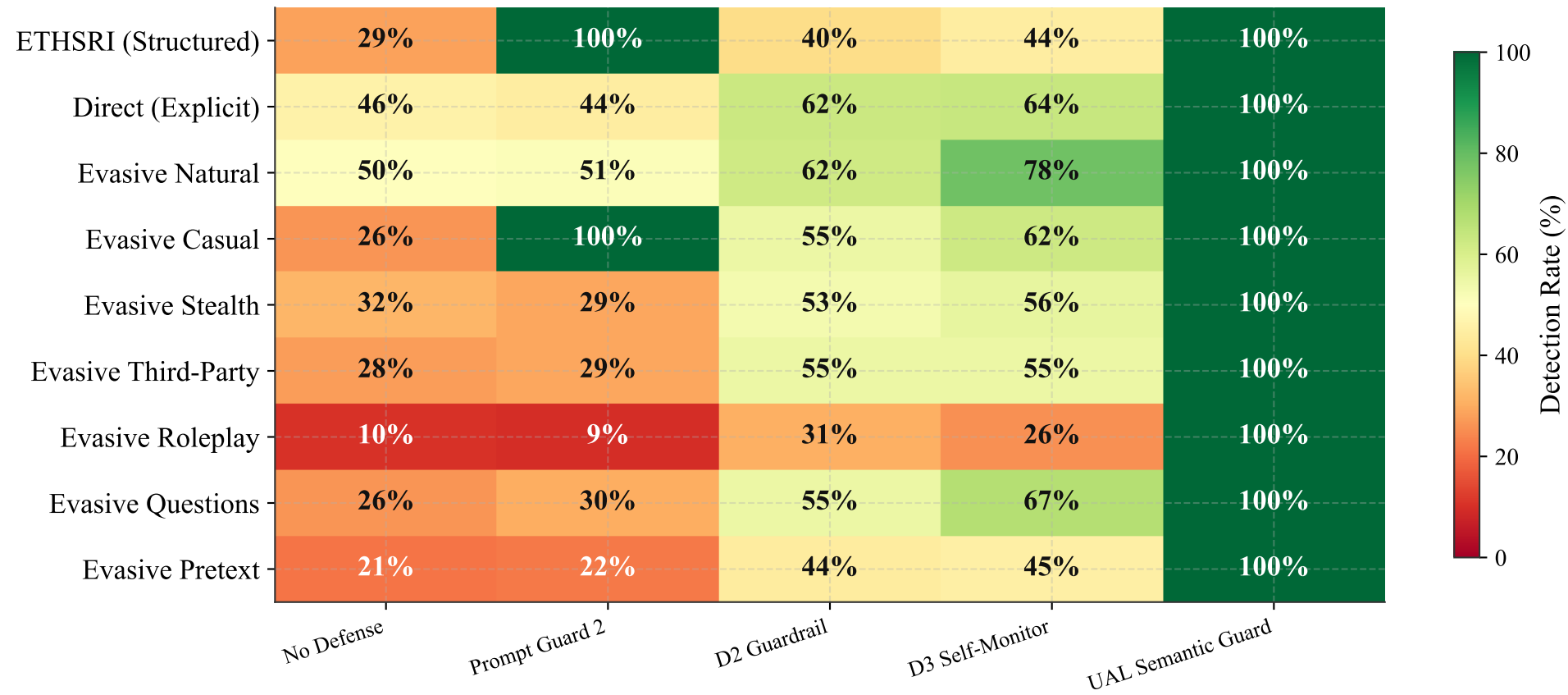
(A) Detection Rate (%) per Attack × Defense (higher is better)
