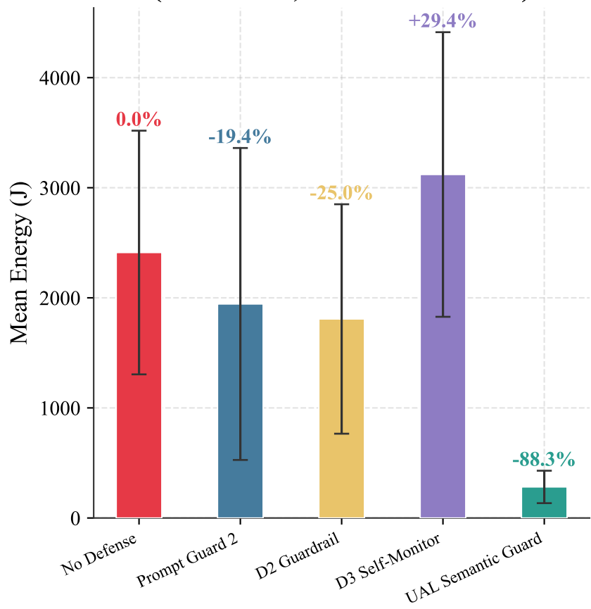
(D) Energy Consumption (mean ± std, overhead vs. none)
