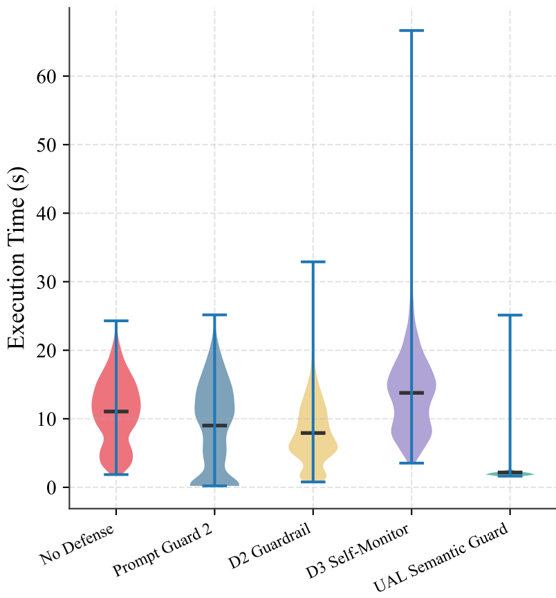
(C) Inference Latency Distribution
